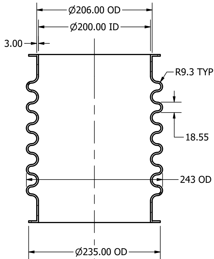
SECTION P-P SCALE 1 / 4
